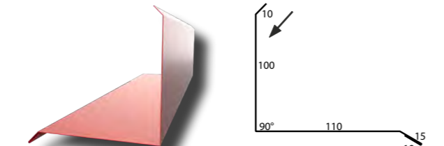
14. ecoORTGANG
