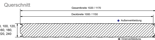
PWS2-MW-ST Wand Standard
